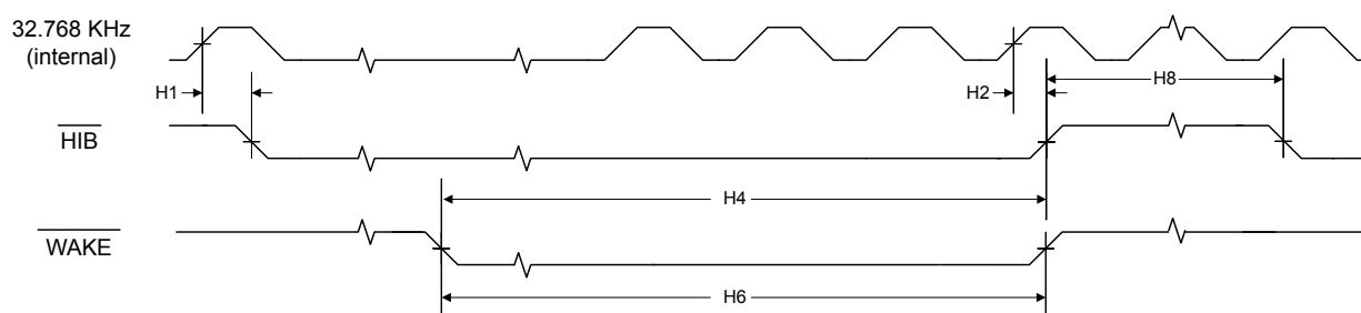
Figure 26-15. Hibernation Module Timing with Internal Oscillator Stopped in Hibernation
